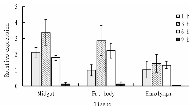
Fig. 4 Changes in AaHsp90 expression in different tissues of Antheraea assama after starvation for different time
